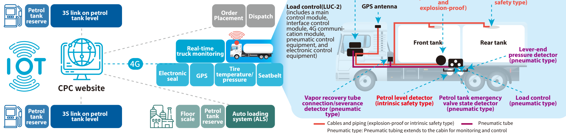
Diagram of the electronicized IoT management system and smart tank truck
